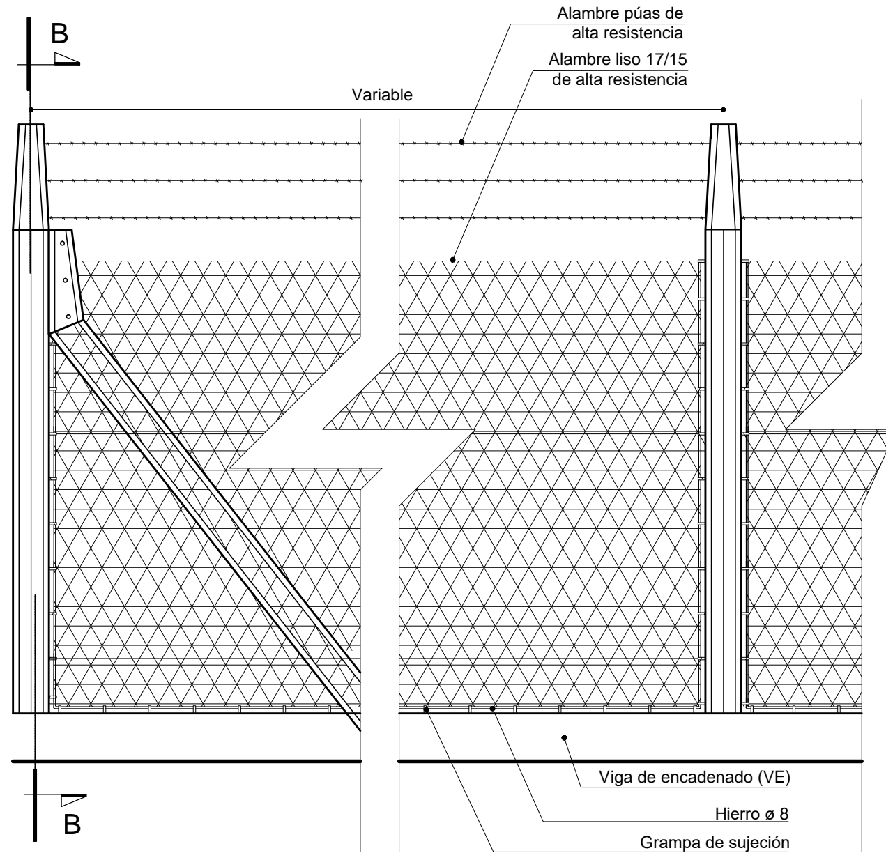
VISTA FRONTAL
